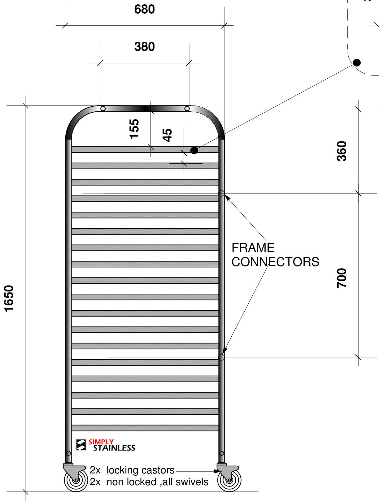
SIDE ELEVATION
