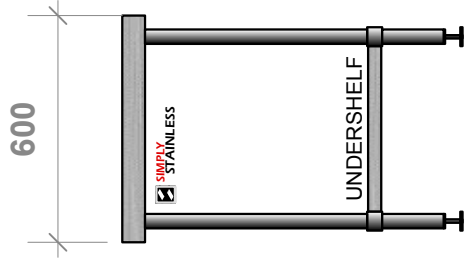
SIDE ELEVATION
