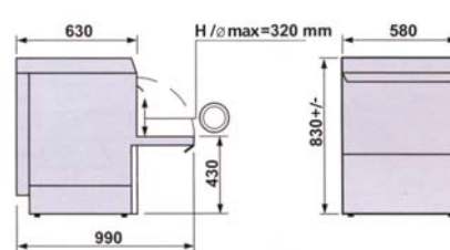
DISHWASHER ecomax 500
