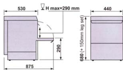
GLASSWASHER ecomax 400-17
